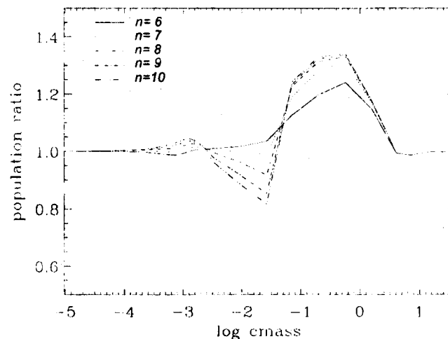
FIGURE 3 Same as Figure 2 but for 6 \leq n \leq 10 .
