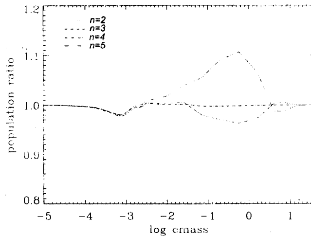
FIGURE 2 The ratio of the population of excited hydrogen-atom states determined with and without processes (1a), (1b), (2a) and (2b) for n \leq 5 , as functions of \log c_{\text{mass}} .
